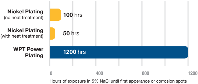
WPT Power FMCP Plating Salt Spray Test
