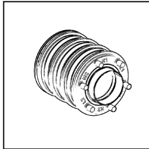
753257 3-way Slip Ring w/ isolation bush, 150mm OD, 30mm
