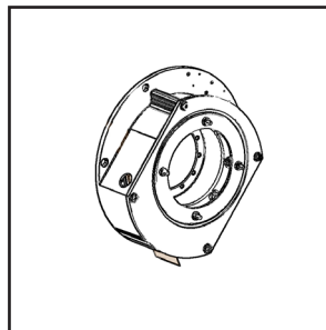
753538 5-way HYAC Assembly with cover
