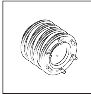
753895 3-144-20 Slip Ring Only, No Earth Ring (8.5° offset)
