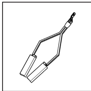
753962 Contact Brush Assembly 65% Ag (yellow) Brush Holder
