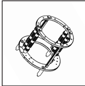
753938 Cage Assembly
