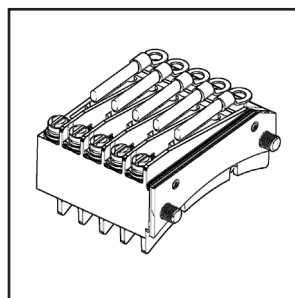
753543 40A Brush Packet
