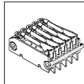
753557 Moulded Brush Pack Assembly
