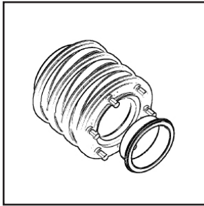
753265 3-144-20 Slip Ring, ISO bush, No Earth Ring (8.5° offset)
