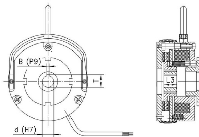
Geared bushing hole diameters
