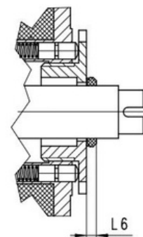
Adjustment nut with a hole and a sealing ring
