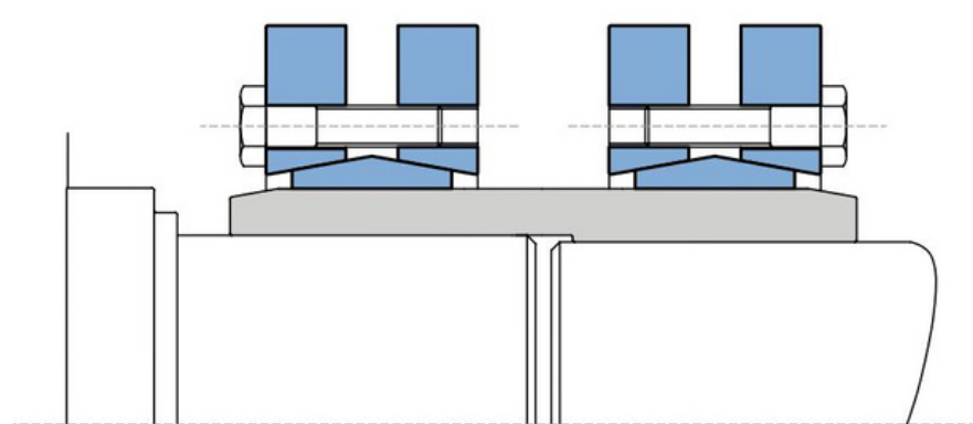
Use of model TLK 603 as coupling between different size shafts
