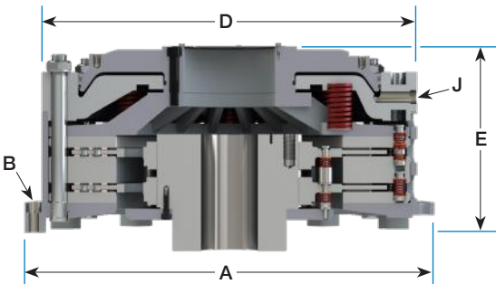
Vertical Mount
